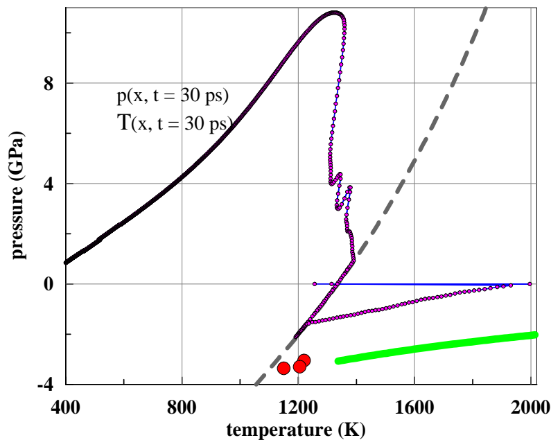
Figure 44. Instant pressure–temperature profile near the moment of time corresponding to the maximum stretching. The red circles, green curve, and melting grey dashed curve are the same as in figure 43. The instant 2T-HD profile is shown by the curve with the small circles on it. This is the run with parameters F_{\text{abs}} = 100 \text{ mJ/cm}^2 , K_{\alpha} = 4 . It is shown in figures 41 and 42. The small circles correspond to the Lagrangian steps (or points) in the finite-difference scheme. There are two evaporated points belonging to the zero pressure level p = 0 .
