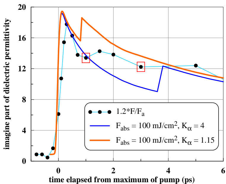
Figure 52. Melting even better is seen in the temporal history \epsilon_2(t) of the imagine part of dielectric function.
