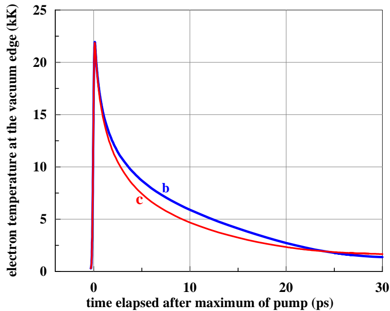
Figure 22. Stronger coupling faster transfers electron energy E_e into ion energy E_i . Thus the conductive time is shorter in the case “c” ( K_\alpha = 1.15 ) than in the case “b” ( K_\alpha = 4 ), and the heat affected zone d_T is thinner, then final equilibrium temperature T \approx T_i \approx T_e is larger in “c”, and ablation threshold is smaller in “c”. Maximum T_e in the moment t \approx 100 fs is achieved at the end of a pump with duration \tau_L = 100 fs for all three case “a”, “b”, and “c” in figure 21.
