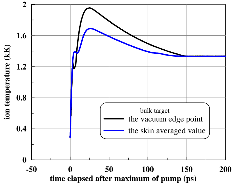
Figure 25. Difference in ion temperatures between the edge value and the skin averaged value. This is a bulk target, F_{\text{abs}} = 100 \text{ mJ/cm}^2 , K_{\alpha} = 4 . After t \approx 150 \text{ ps} the skin returns to the triple point with melting temperature 1.337 kK.
