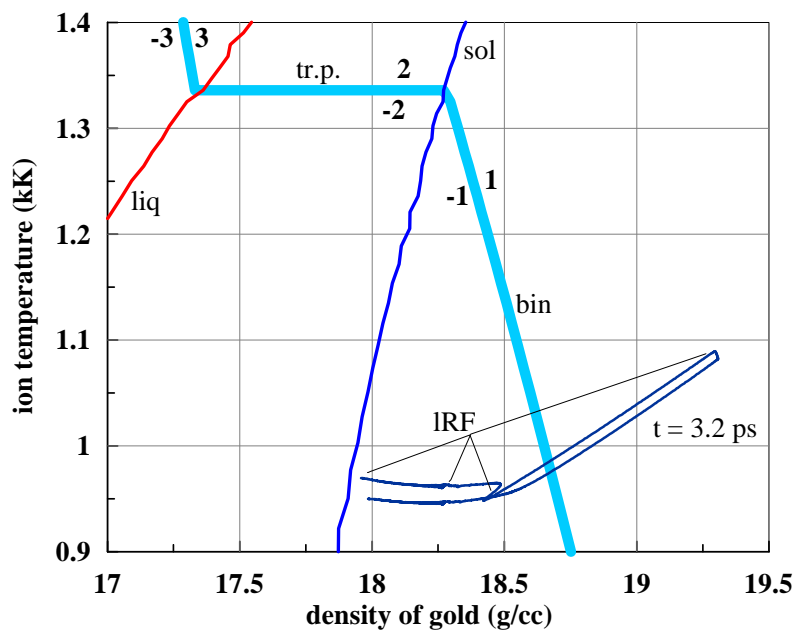
Figure 31. Instant distribution of ion temperature T_i(\rho; t = 3.2 ps) across a film shown at the phase diagram; d_f = 30 nm, F_{abs} = 32 mJ/cm 2 , 0.55 MJ/kg. The distribution repeats the profile in figure 29 with its left (IRF) and right (rRF) wings. Even the trace 1–2–3 is seen well in the left wing. The pairs of digits 1–1, 2–2 and 3–3 relate to stable and metastable states of solid, solid–liquid mixture, and liquid respectively. The stable and metastable states are separated by the binodal curve “bin”. Other designation are the same as in figure 18.
