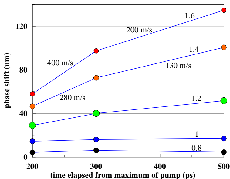
Figure 50. Late stage deceleration according to pump-probe measurements. The digits give normalized fluence F/F_a . There are three experimental points covering the temporal range from 200 to 500 ps. Expansion velocities found from the spatiotemporal positions of the filled circles are given for the upper two curves.
