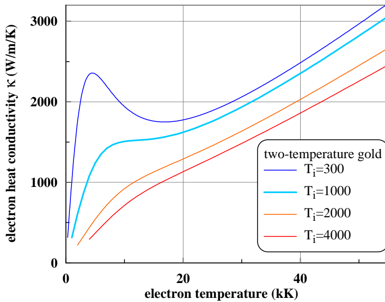
Figure C1. Variation of a 2T heat conduction coefficient \kappa(\rho, T_e, T_i) with temperatures T_e and T_i in isochorically heated solid density \rho_0 gold.
