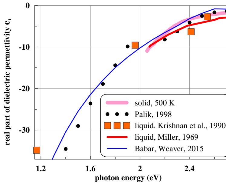
Figure D4. Influence of heating and melting on e_1(E) . The curves “Palik” [87] and “Babar, Weaver” [18] relate to room temperature. The curves “Miller” [24] and “Krishnan” [25] correspond to liquid. Solid heated to 500 K is also shown. These data are taken from [24].
