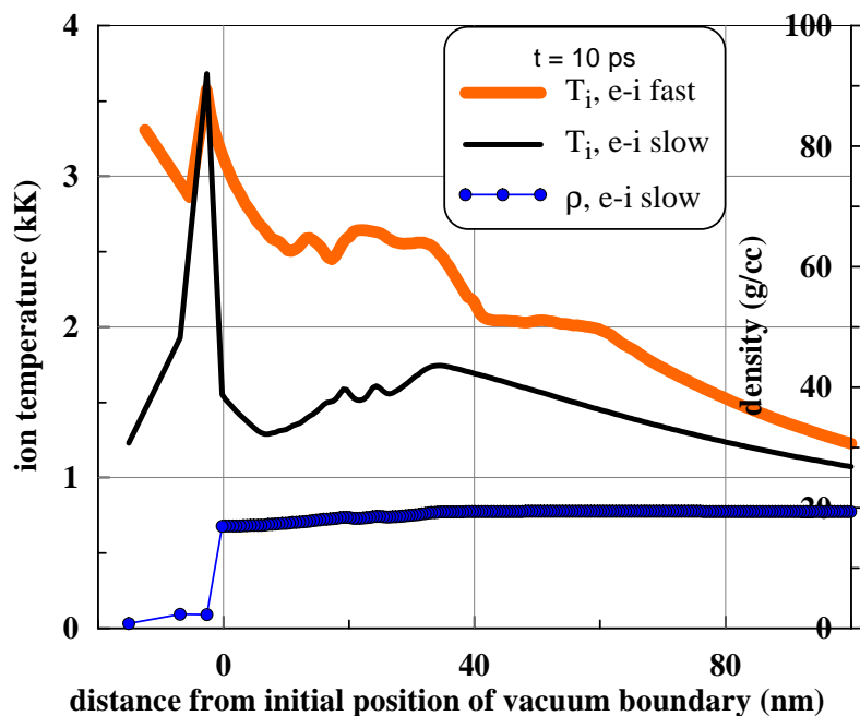
Figure 12. Slow increase of T_i and slow melting in the case with small \alpha . The case with absorbed energy F_{abs} = 100 \text{ mJ/cm}^2 is shown.
