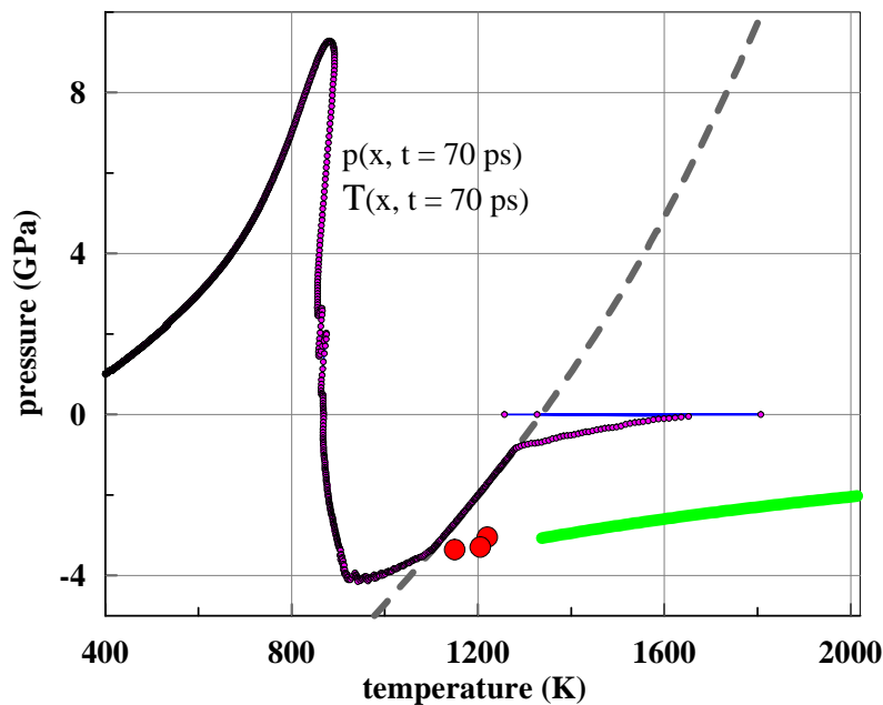
Figure 45. The same profile as in figure 44 but now for the later instant 70 ps. This instant is after the instant when the maximum (in time evolution) tensile stress p_{xt*} is achieved. After that the maximum in space stress p_{x*} at the current instant profile is approximately equal to the value p_{xt*} . The value p_{x*} slowly decreases on a long time interval.
