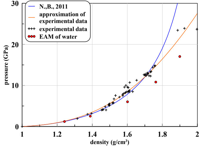
Figure 19: Comparison of EoS [51] with experimental data on shock compression from [16, 17]. We also compare with experiment the Hugoniot adiabetic curve following from the EAM potential for water used in simulations ## VIII, IX. The abbreviation N.,B., 2011 relates to the paper [51]. Semi-analytic approximation of experimental data is taken from [10, 9]. It is valid from infinitesimal compressions and up to 120 GPa - the highest measured pressures.
