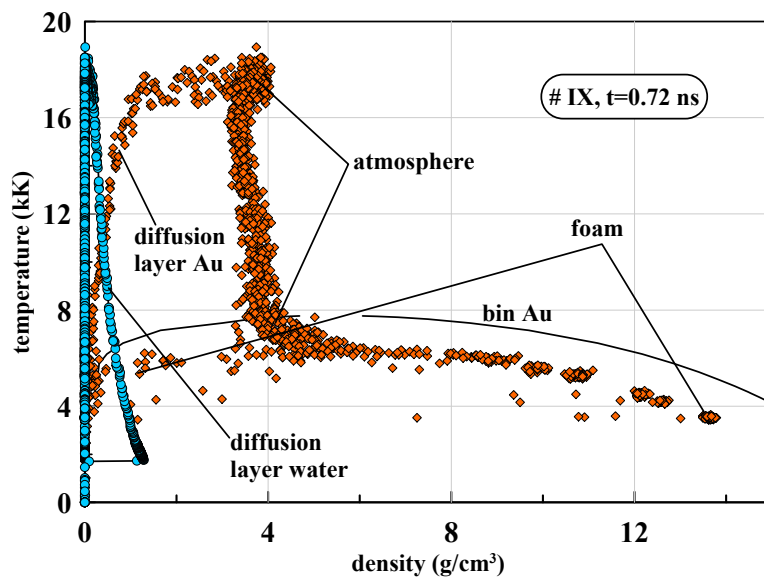
Figure 13: Instant density \rho(x, t) and temperature T(x, t) profiles for t = 0.72 ns plotted excluding dependence on x as a parametric function T(\rho, t = 0.72) at a phase diagram of gold. The orange rhombuses correspond to gold, the blue circles correspond to water.
